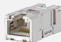
E-DAT Industry RJ45 coupler insert 1401200810MI
